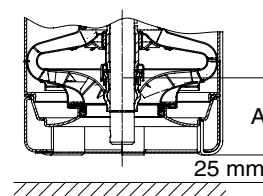
Obr. 20 MTR(E) 32, 45 a 64
